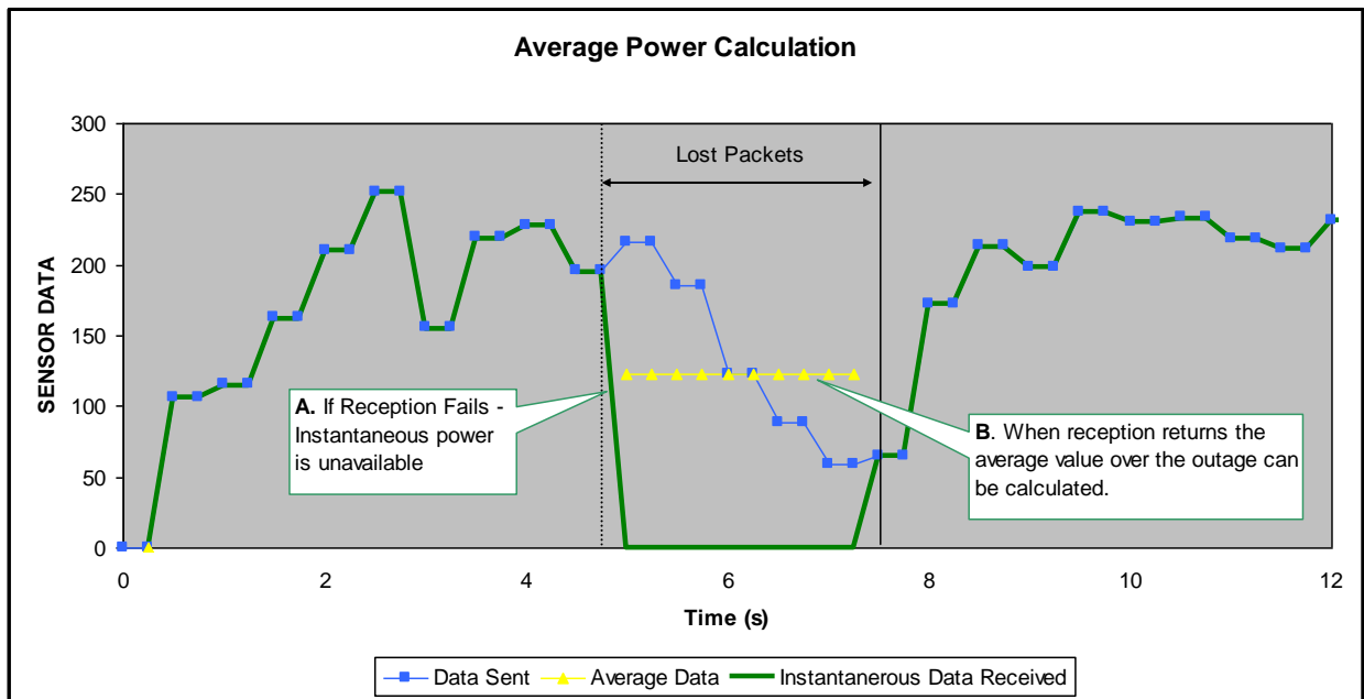
Figure 5-4. Averaging Power through an RF Outage
