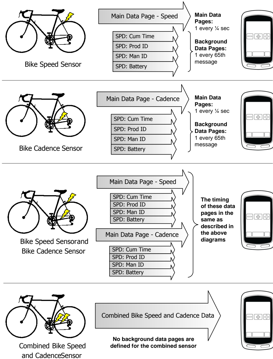
Figure 4-3. ANT+ Bike Speed and Cadence Use Cases and Associated Data Messages
