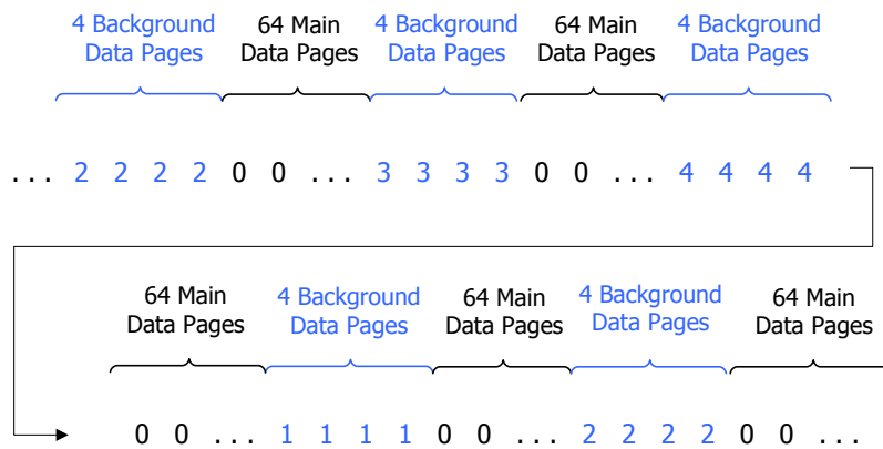
Figure 5-2. Regular Broadcast Transmission Pattern with Optional Data Pages
